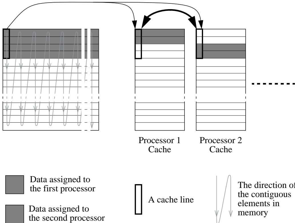
Figure 8-1. False Sharing
